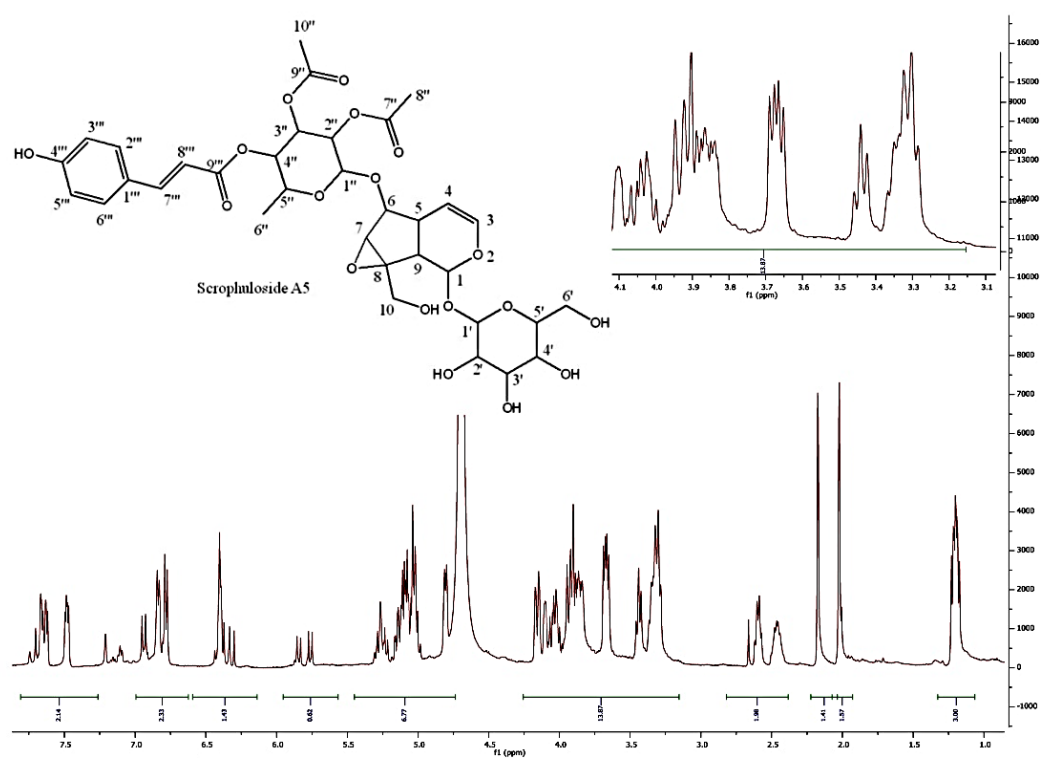
Fig. 11. ^1\text{H} -NMR spectrum of scrophuloside A5, 500 MHz, DMSO-D6
