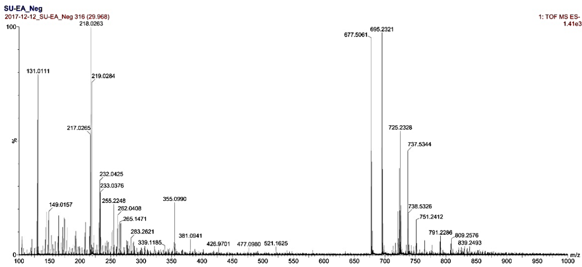
Fig. 4. UHPLC-MS-QTOF spectrum scrophuloide A6 (6) on negative mode
