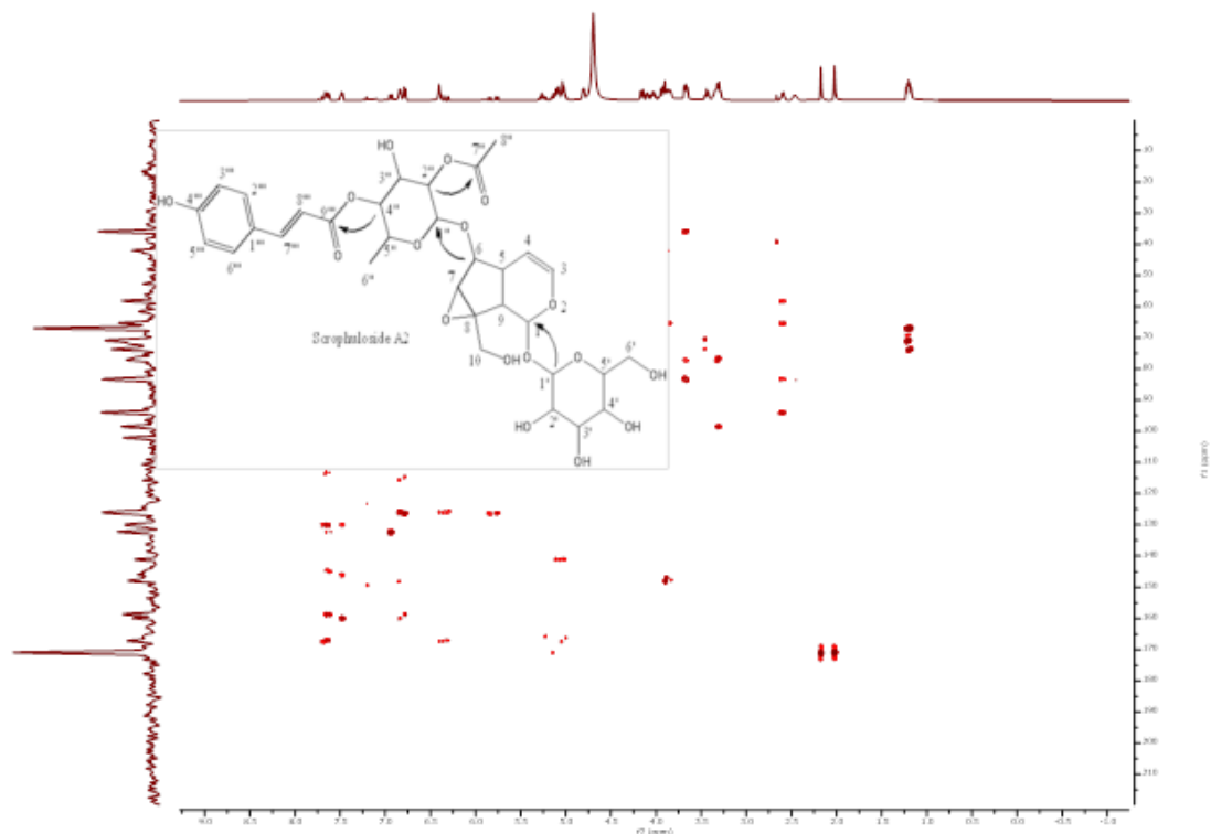
Fig. 7. HMBC spectrum of scrophuloside A2, 500 MHz, DMSO-D6
