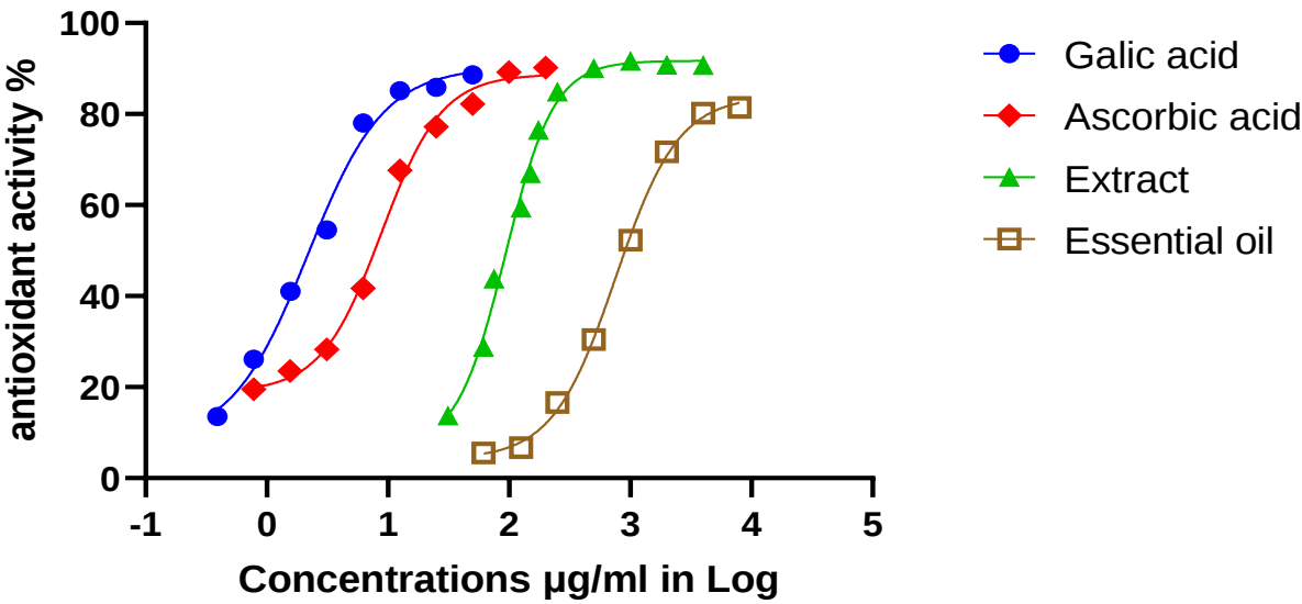
Fig. 1. Scavenging effect of the essential oil and the methanol extract of N. crisper on DPPH free radical
