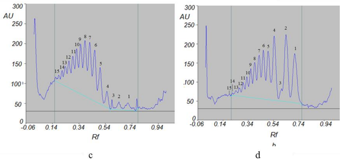
Fig. 3. a) TLC analysis of inulin in visible mode (1. extracted inulin, 2. sigma standard, 3. fiber rific standard, 4. fructose, 5. sucrose); b) TLC analysis of inulin in fluorescence mode (1. fiber rific standard, 2. extracted inulin); c) TLC analysis of fiberrific standard in fluorescence mode (1. fructose, 2. sucrose, 3. 1- kestose, 4. Nystose and 5-15. Oligomers (DP = 5-15)); d) TLC analysis of extracted inulin in fluorescence mode (1. fructose, 2. sucrose, 3. 1- kestose, 4. Nystose and 5-15. Oligomers (DP = 5-15))
