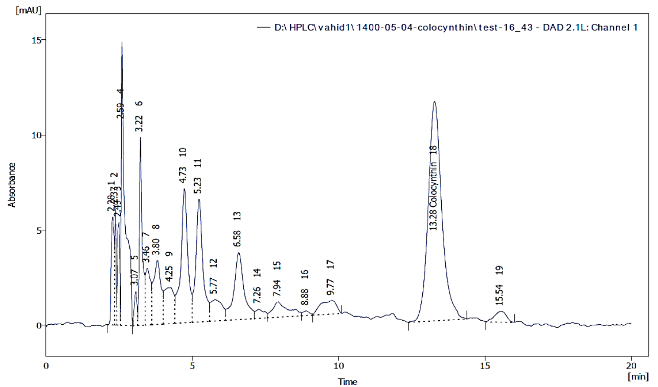
Fig. 1. HPLC Chromatogram of fruit pulp extract of C. colocynthis
