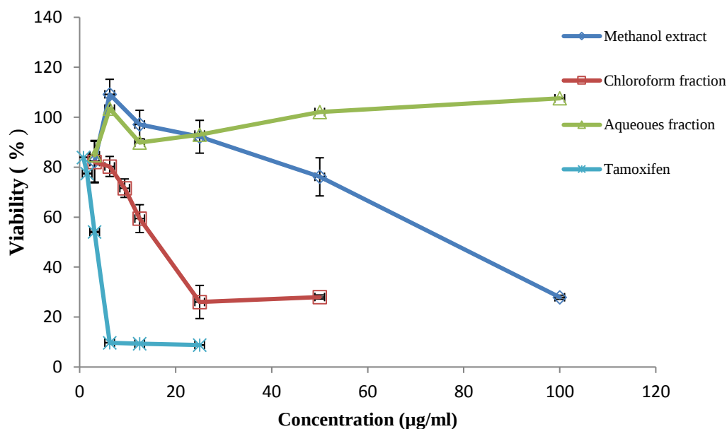
Fig. 1. Cytotoxic effects of C. albonitens extract and fractions in MCF-7 cells
