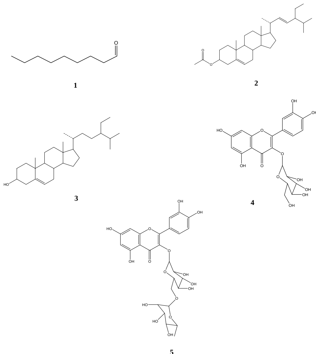
Figure 1- Structures of the isolated compounds from L. staurophyllum
