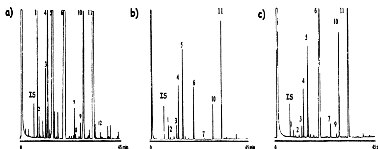
Fig. 4. Chromatograms of the SWE (a), dichloromethane extraction (b) and hydrodistillation (c) of fennel essential oil. Peaks identification: (1) \alpha -pinene; (2) \beta -pinene; (3) \beta -myrcene; (4) \alpha -phellandrene; (5) limonene; (6) unknown; (7) camphor; (8) terpinen-4-ol; (9) linalyl propanoate; (10) unknown; (11) anethol; (12): copaene.
