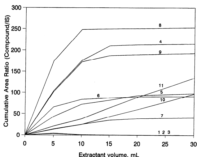
Fig. 2. Kinetic curves obtained by SWCE under optimum working conditions for (1) \alpha -pinene; (2) \beta -pinene; (3) \beta -myrcene; (4) eucalyptol; (5) linalool; (6) 2-methyl-6-methylen-7-octen-2-ol; (7) terpinen-4-ol; (8) \alpha -terpineol; (9) geraniol; (10) geranyl acetate and (11) 4-ethenyl- \alpha,\alpha , 4-trimethyl-3-(1-methylethenyl) cyclohexanemethanol (11). Eucalyptol peaks were divided by 8 in order to fit them into the scale.
