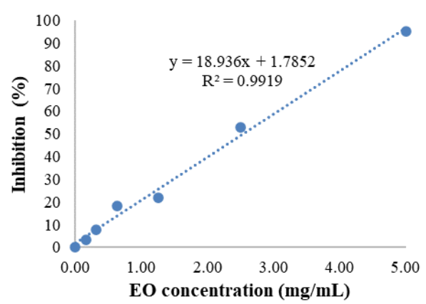
Fig. 7. The Ferric reducing antioxidant power (FRAP) of EO
