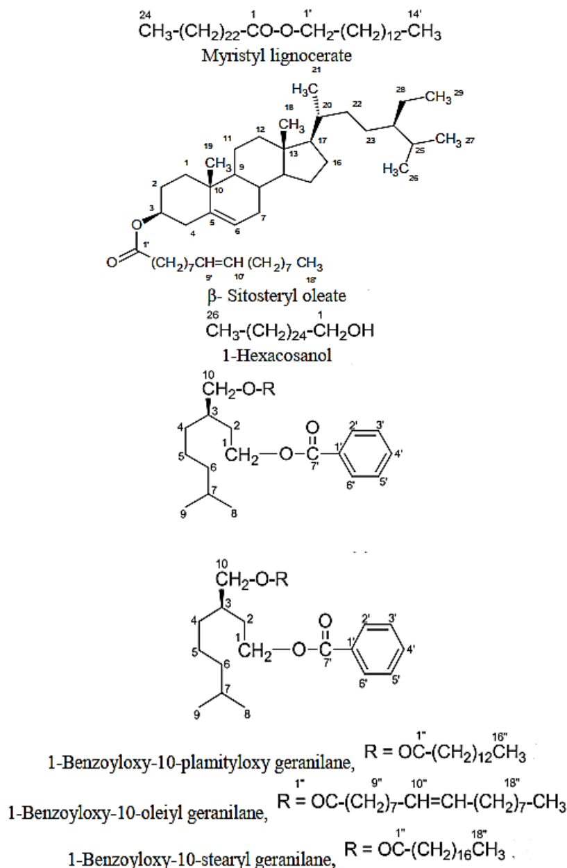
Fig. 3. Compound isolated from root bark of P. mollissima [33]
