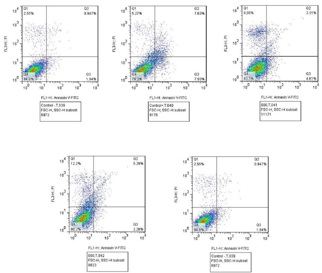
Fig. 3. Verification of apoptotic and necrotic cell death using the standard method of flow cytometry; a) untreated prostate PC-3 cells, b) treated prostate PC-3 cells on day 3 (oil doses of 800 \mu g/ml)
