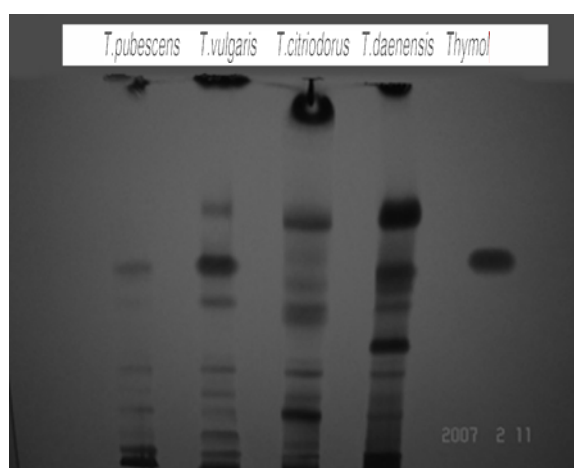
Fig. 1- TLC chromatogram of dichloromethane extract of Thymus spp.
