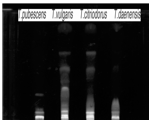
Fig. 2- TLC chromatogram of ethylacetate extract of Thymus spp.
