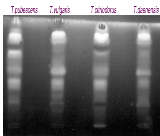
Fig. 3- TLC chromatogram of n -butanol extract of Thymus spp
