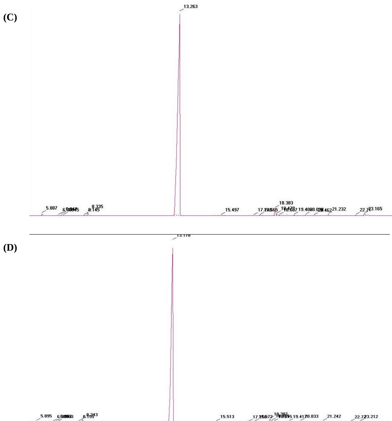
Fig. 3- Sample chromatograms of GC-FID of essential oil isolated from Ocimum basilicum L. aerial parts in treatments of (A): Control as soil without sewage sludge and irradiation; (B): 15 g kg -1 of sewage sludge irradiated with 20 kGy; (C): 30 g kg -1 of sewage sludge irradiated with 20 kGy; (D): 60 g kg -1 of sewage sludge irradiated with 20 kGy
